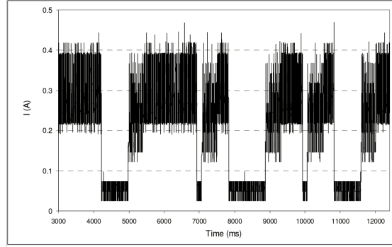
Figure 3.8: Sample measurement of TX-Power technique
