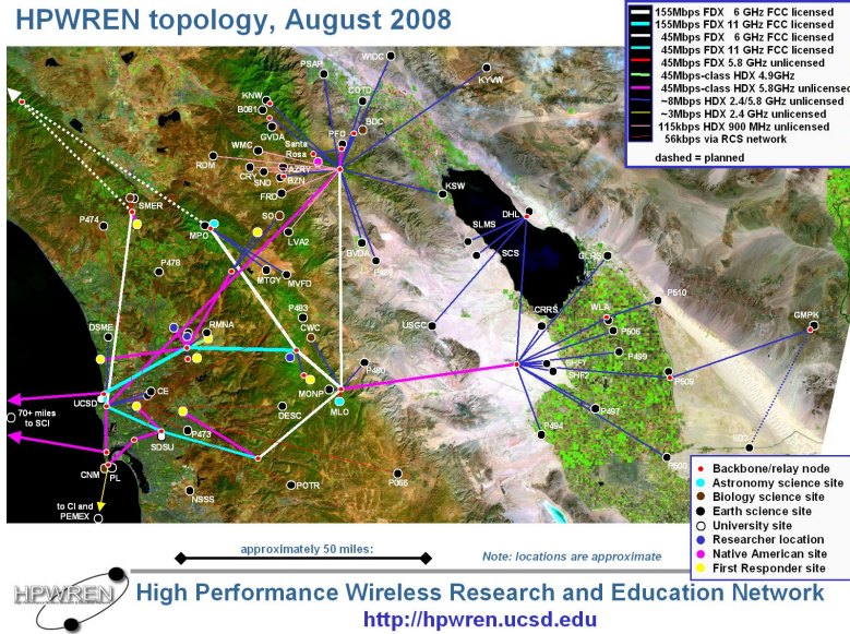
Figure 1.1: HPWREN: network topology
