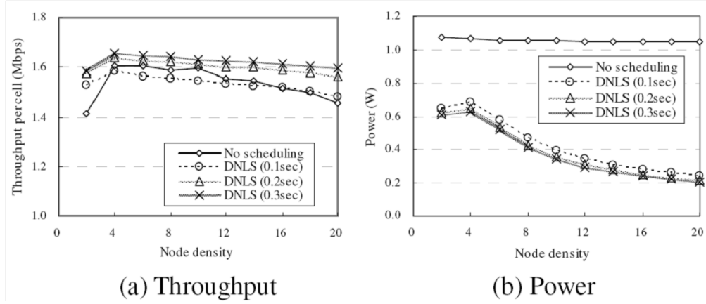
Figure 3.5: Simulation results of the node-level scheduling algorithm in hexagonal topology using different slot sizes
