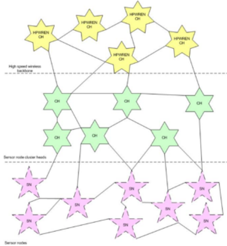
Figure 1.2: HPWREN: three layer structure
