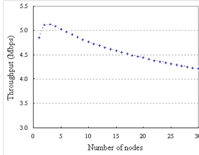
Figure 3.1: Throughput drop as a function of the number of nodes transmitting at full MAC queues
