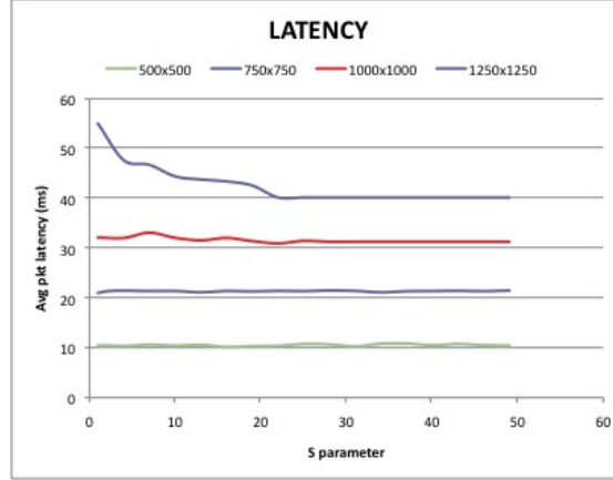
Figure 5.3: Average latency (ms) as a function of the S parameter of the algorithm for different square networks with sides 500m, 750m, 1000m and 1250m
