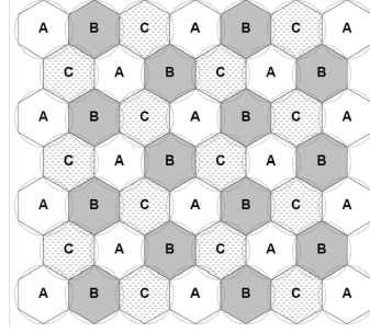
Figure 3.3: Hexagonal network topology used in the simulations for the scheduling algorithm
