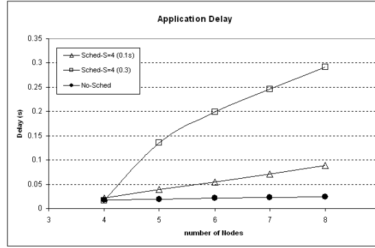
Figure 3.9: Measurement results on application layer delay
