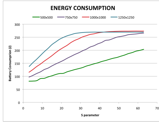
Figure 5.1: Average per node battery consumption (J) as a function of the S parameter.
