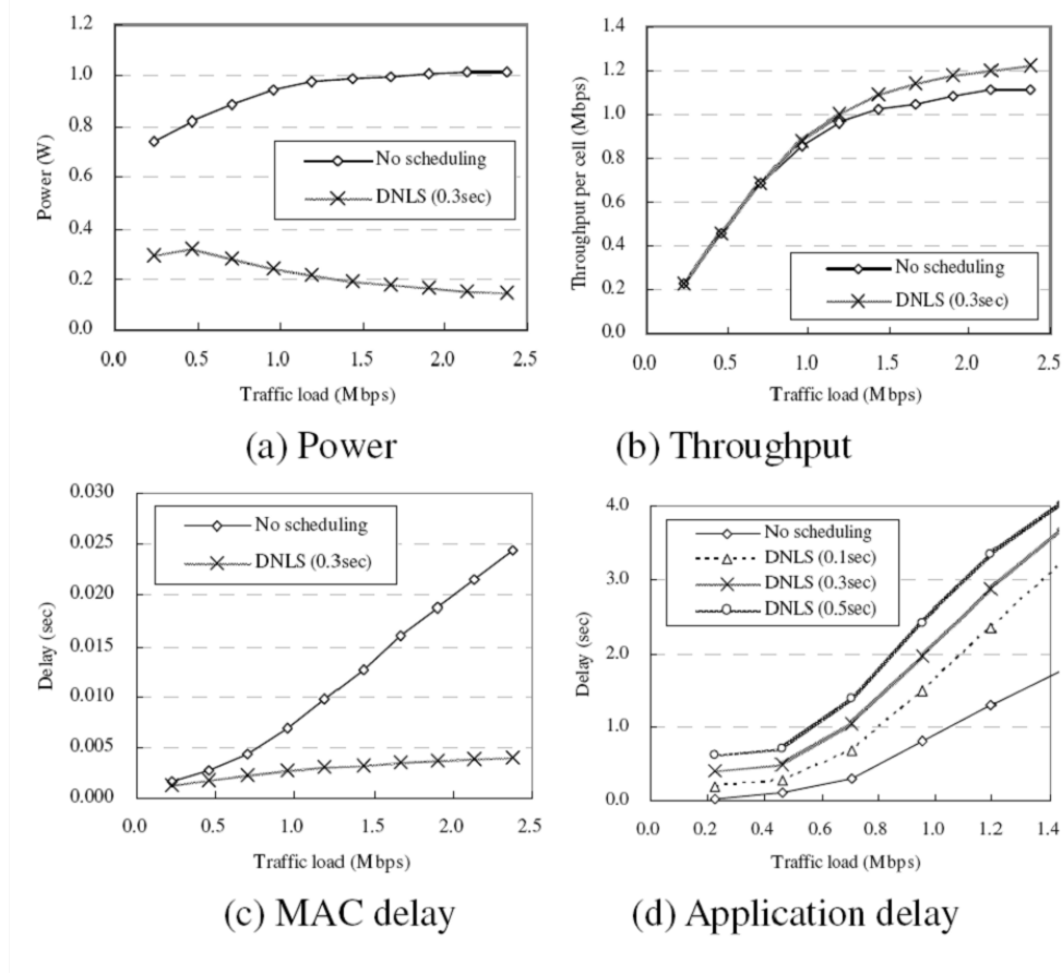
Figure 3.4: Simulation results of the node-level scheduling algorithm in hexagonal topology using data collected from HPWREN
