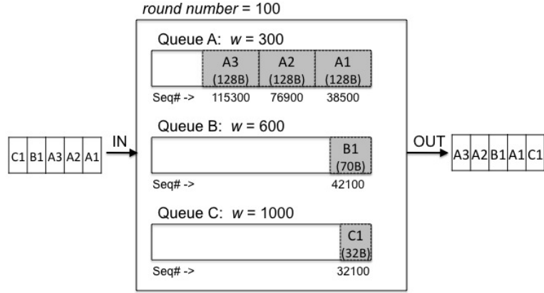
Figure 3.10: Example of the WFQ policy implemented at node level
